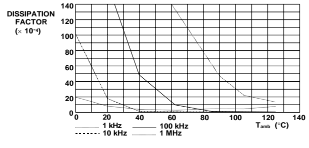
Typical dissipation factor as a function of temperature and frequency
